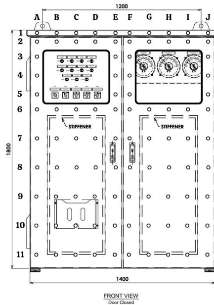
FRONT VIEW Door Closed
